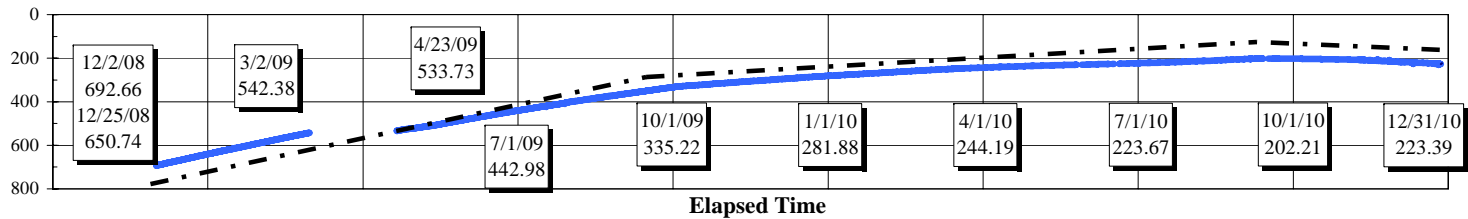
Calculated Water Level in Well (fbs)
